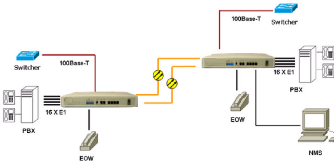
Fig 1-3-1 Point to Point Application
