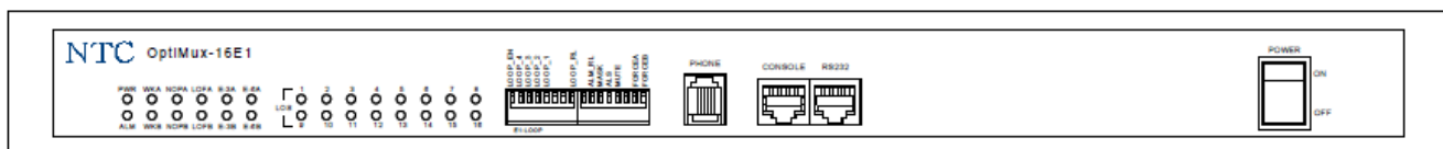
Fig 3-1-1 Front Panel (16E1)
